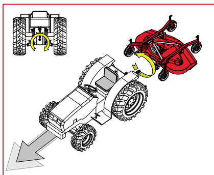
CONFIGURATION 1. Finishing mowers: rear Rotation of tractor's PTO: CLOCKWISE (standard) Advancing direction: front
