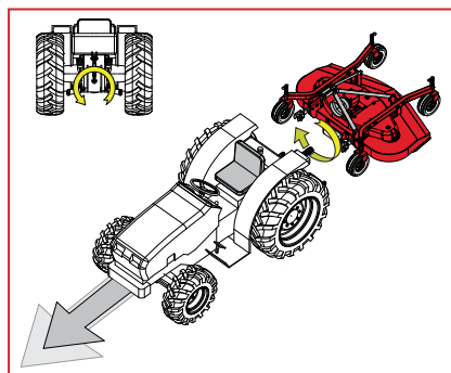
CONFIGURATION 2. Finishing mowers: rear Rotation of tractor's PTO: COUNTERCLOCKWISE Advancing direction: front
