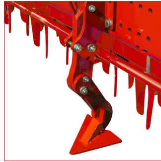
Pair of track eradicator tines with shear bolt
